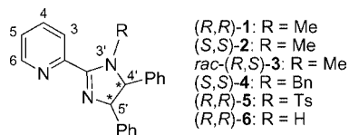
Figure 2. 2-(4',5'-Diphenyl-3'-R-imidazolyl)pyridines 1–6 with numbering scheme.
