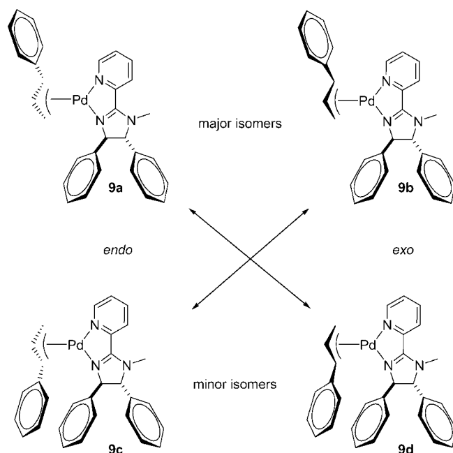
Figure 4. Proposed structures for the four isomers of 9 observed in solution (arrows indicate the isomer interconversion observed by 2D NOESY, between 9a and 9d , and 9b and 9c ).
