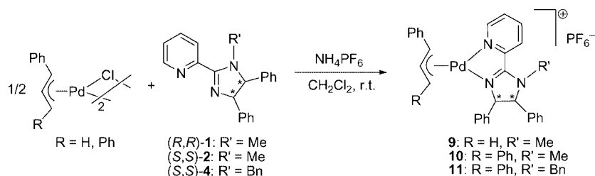
Scheme 1. Allylpalladium complexes 9–11 containing chiral ligands (R,R) - 1 , (S,S) - 2 and (S,S) - 4 .
