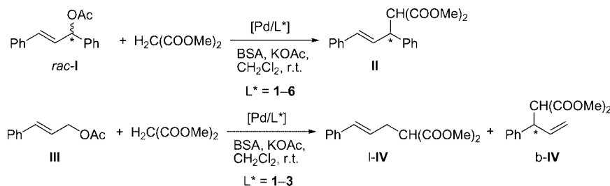
Scheme 2. Allylic alkylation of rac - I and III catalysed by \text{Pd}/\text{L}^* systems ( \text{L}^* = \mathbf{1-6} ).
