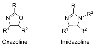
Figure 1. Oxazoline and imidazoline heterocycles.
